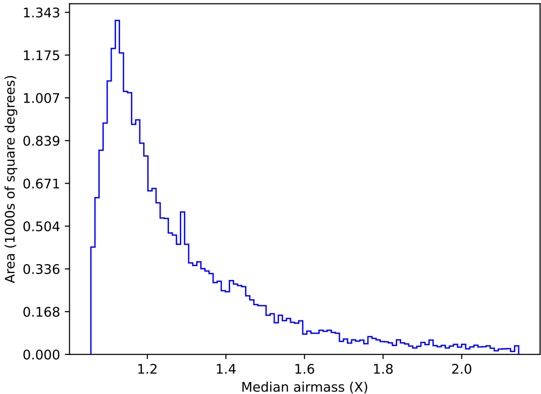
too_elab_r8_d3_ugrizy_v3.4_10yrs Yr 1 g band: Median airmass
