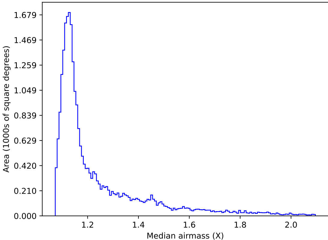
too_elab_r8_d3_ugrizy_v3.4_10yrs Yr 1 all bands: Median airmass
