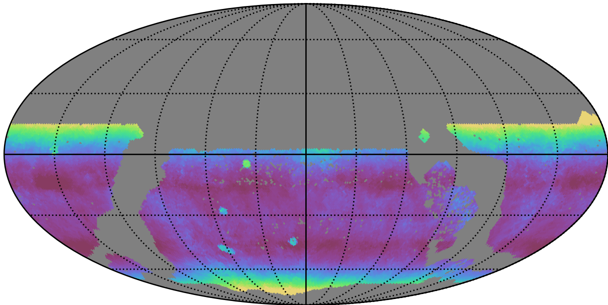
too_elab_r8_d3_ugrizy_v3.4_10yrs WFD y band: Median airmass
