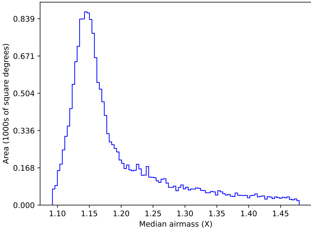
too_elab_r8_d3_ugrizy_v3.4_10yrs WFD y band: Median airmass
