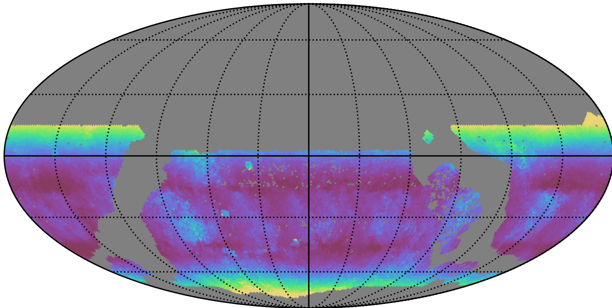
too_elab_r8_d3_ugrizy_v3.4_10yrs WFD u band: Median airmass
