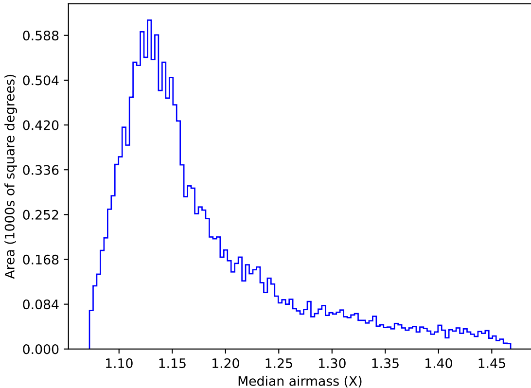
too_elab_r8_d3_ugrizy_v3.4_10yrs WFD u band: Median airmass
