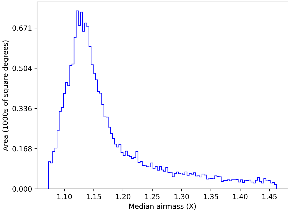
too_elab_r8_d3_ugrizy_v3.4_10yrs WFD r band: Median airmass
