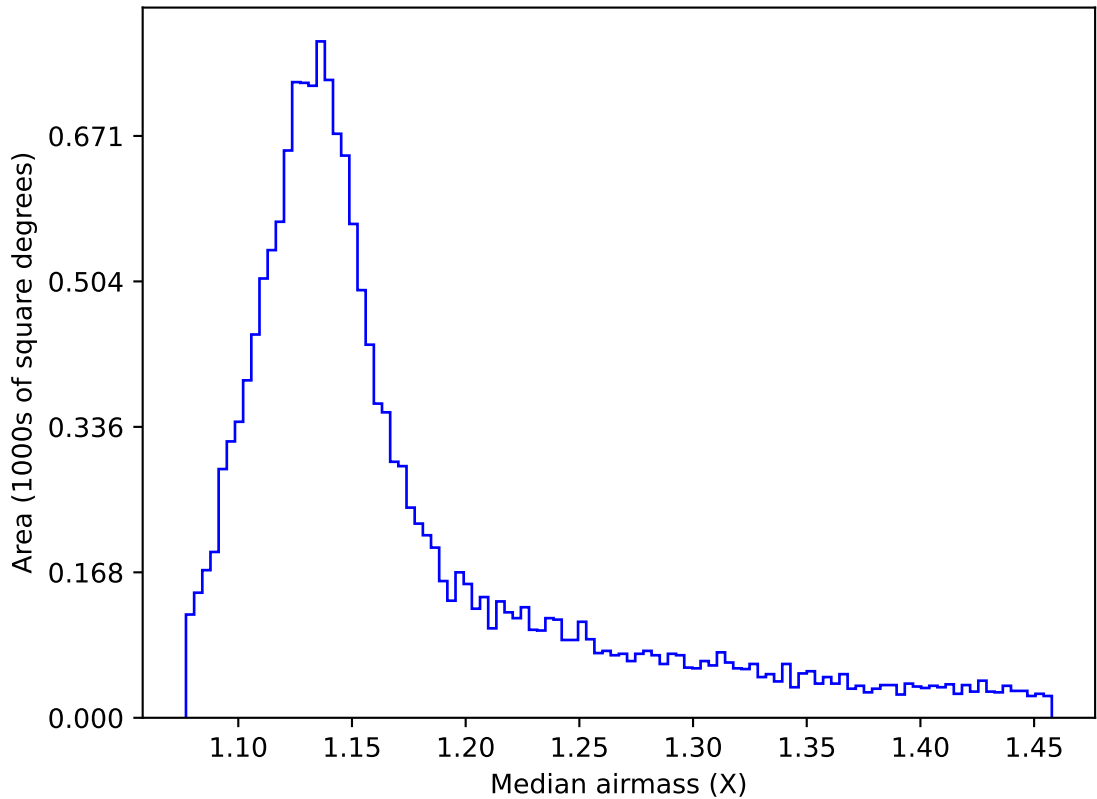
too_elab_r8_d3_ugrizy_v3.4_10yrs WFD i band: Median airmass
