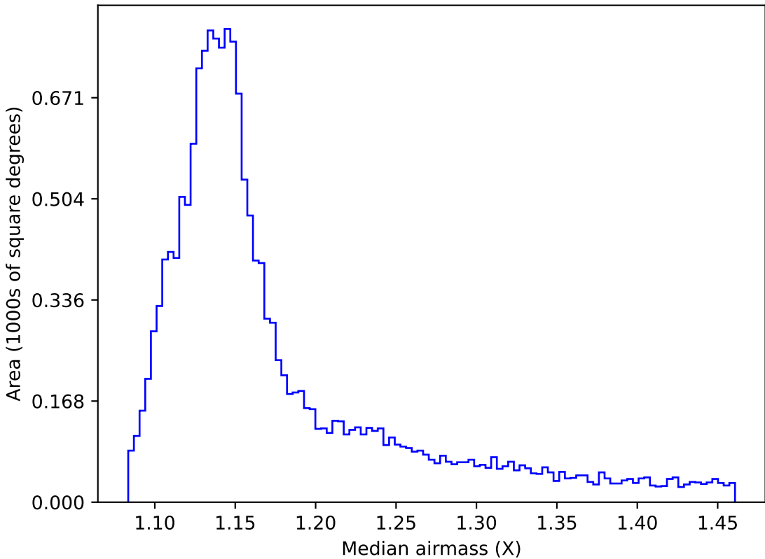
too_elab_r8_d3_ugrizy_v3.4_10yrs WFD all bands: Median airmass
