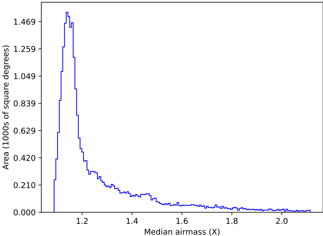
too_elab_r8_d3_ugrizy_v3.4_10yrs All sky z band: Median airmass
