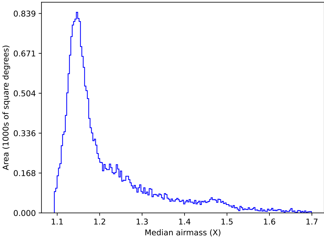
too_elab_r8_d3_ugrizy_v3.4_10yrs All sky y band: Median airmass
