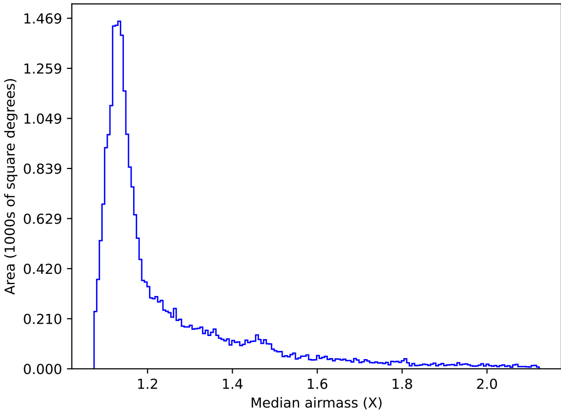
too_elab_r8_d3_ugrizy_v3.4_10yrs All sky r band: Median airmass
