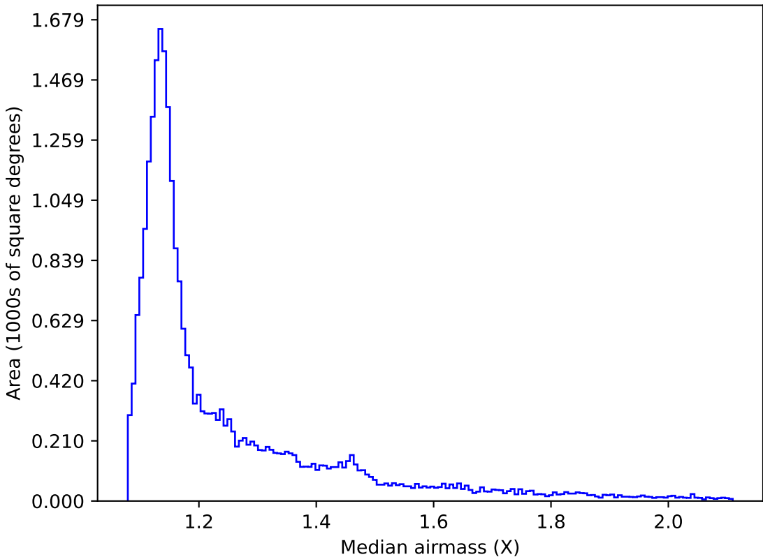
too_elab_r8_d3_ugrizy_v3.4_10yrs All sky i band: Median airmass
