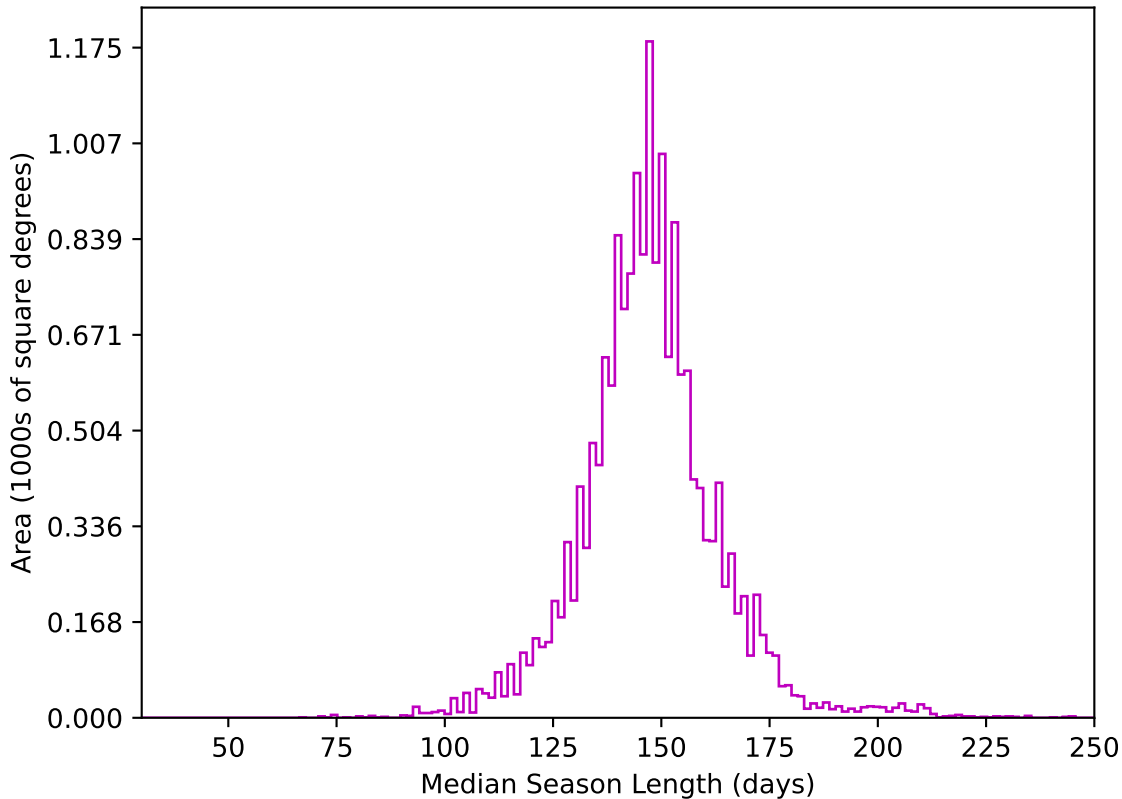
too_elab_r8_d3_ugrizy_v3.4_10yrs WFD z band: Median Season Length
