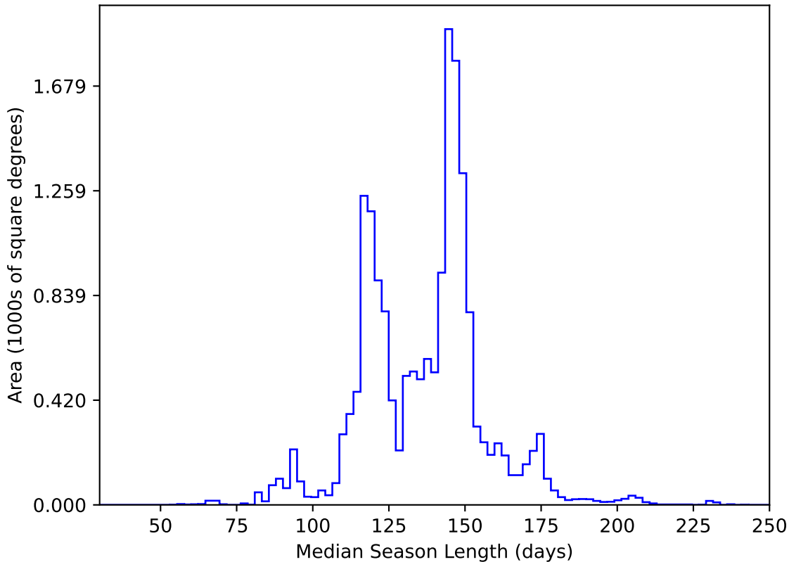
too_elab_r8_d3_ugrizy_v3.4_10yrs WFD y band: Median Season Length
