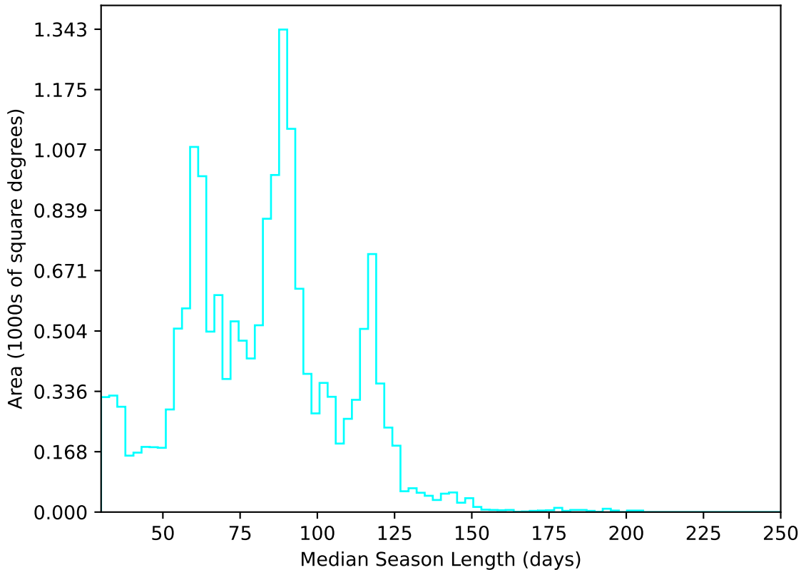
too_elab_r8_d3_ugrizy_v3.4_10yrs WFD u band: Median Season Length
