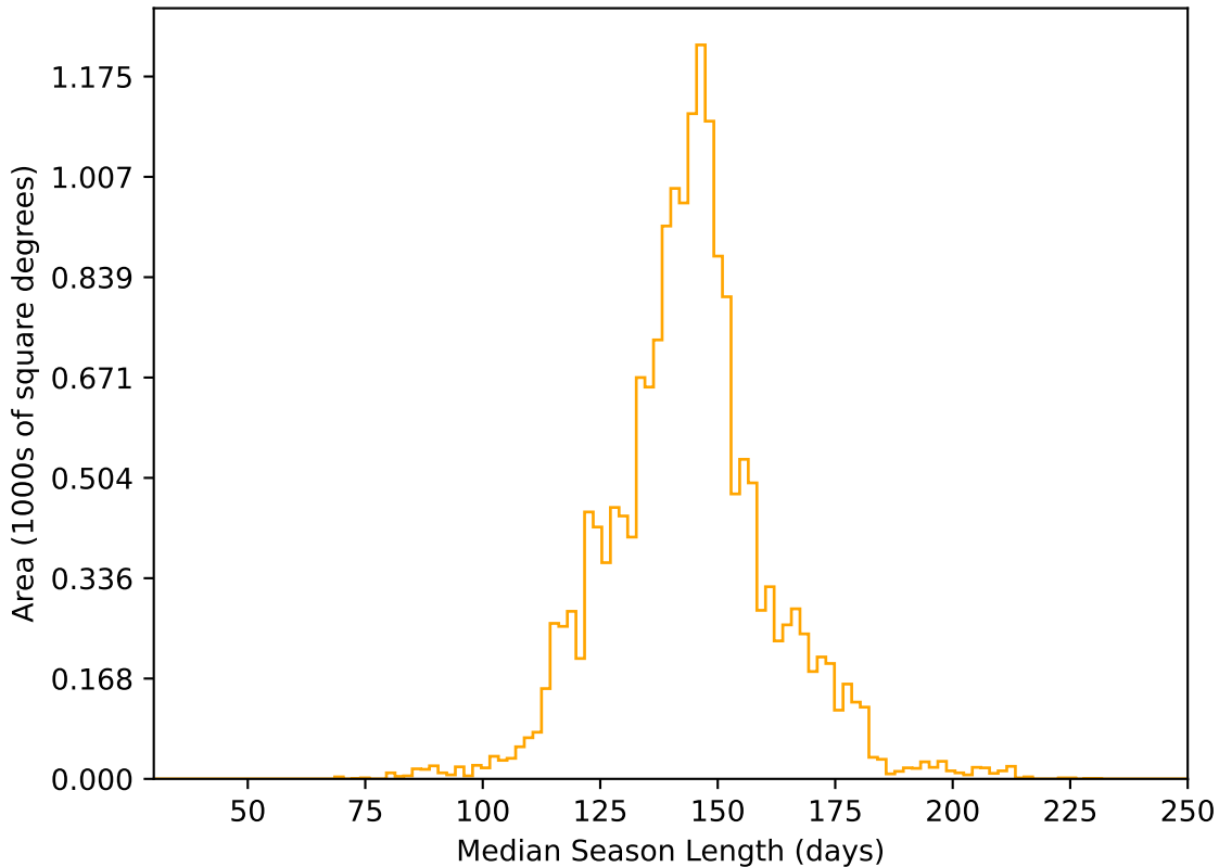
too_elab_r8_d3_ugrizy_v3.4_10yrs WFD r band: Median Season Length
