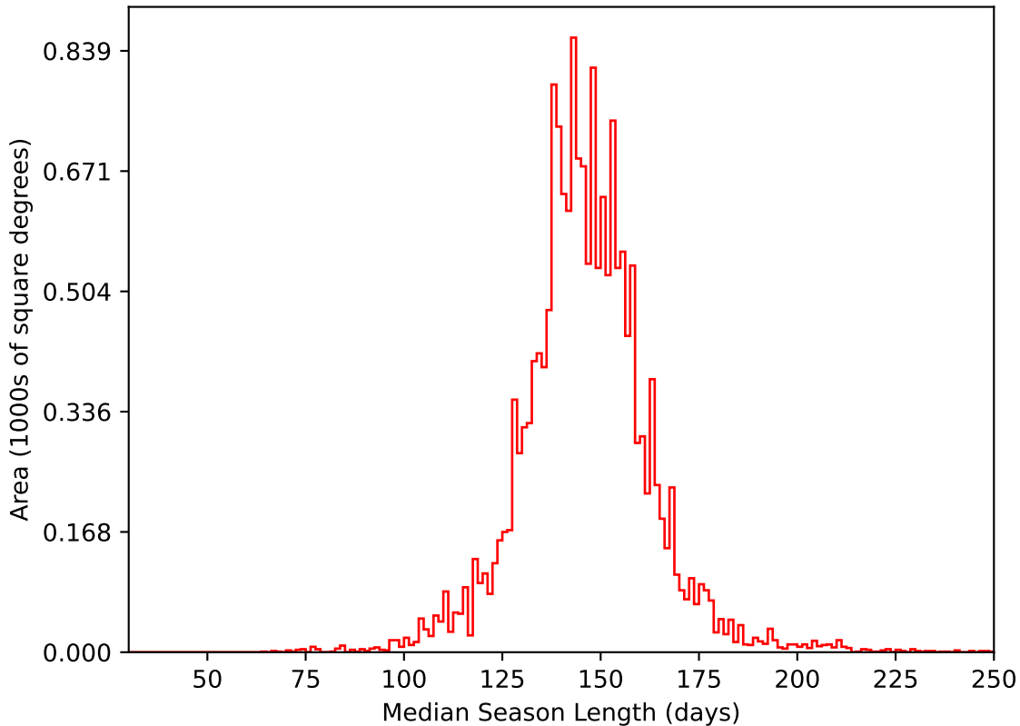
too_elab_r8_d3_ugrizy_v3.4_10yrs WFD i band: Median Season Length
