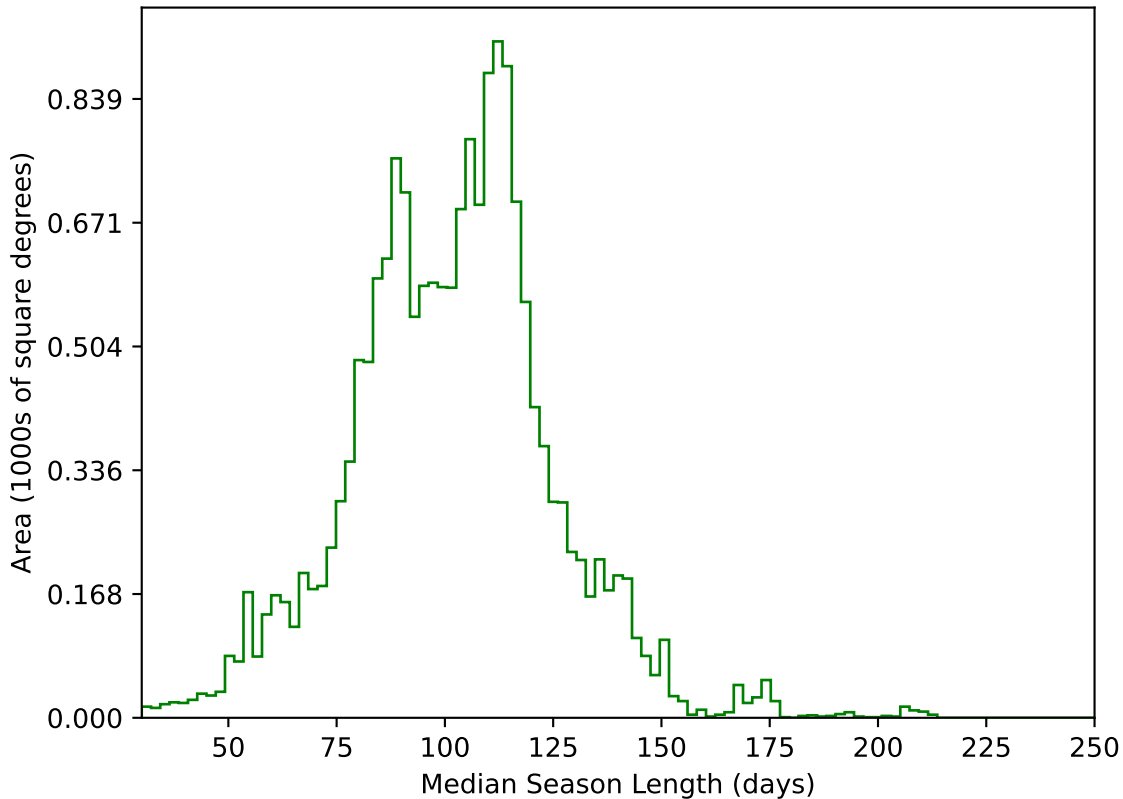
too_elab_r8_d3_ugrizy_v3.4_10yrs WFD g band: Median Season Length
