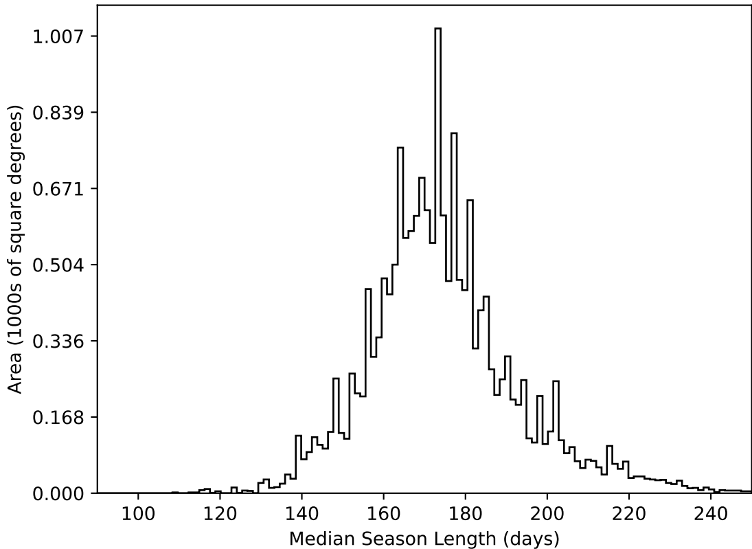
too_elab_r8_d3_ugrizy_v3.4_10yrs WFD all bands: Median Season Length
