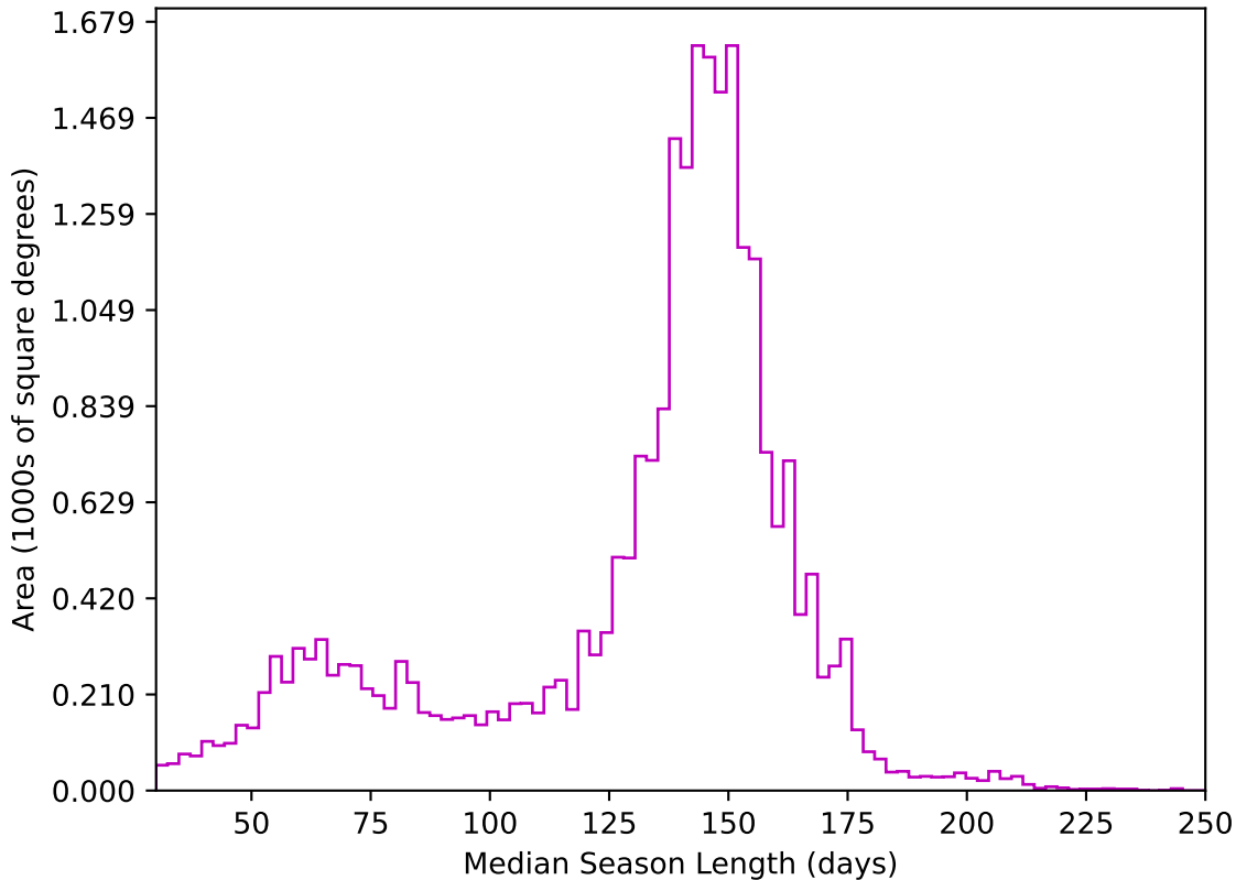
too_elab_r8_d3_ugrizy_v3.4_10yrs All sky z band: Median Season Length
