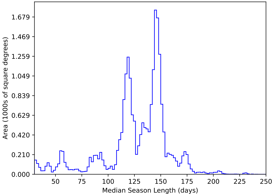
too_elab_r8_d3_ugrizy_v3.4_10yrs All sky y band: Median Season Length
