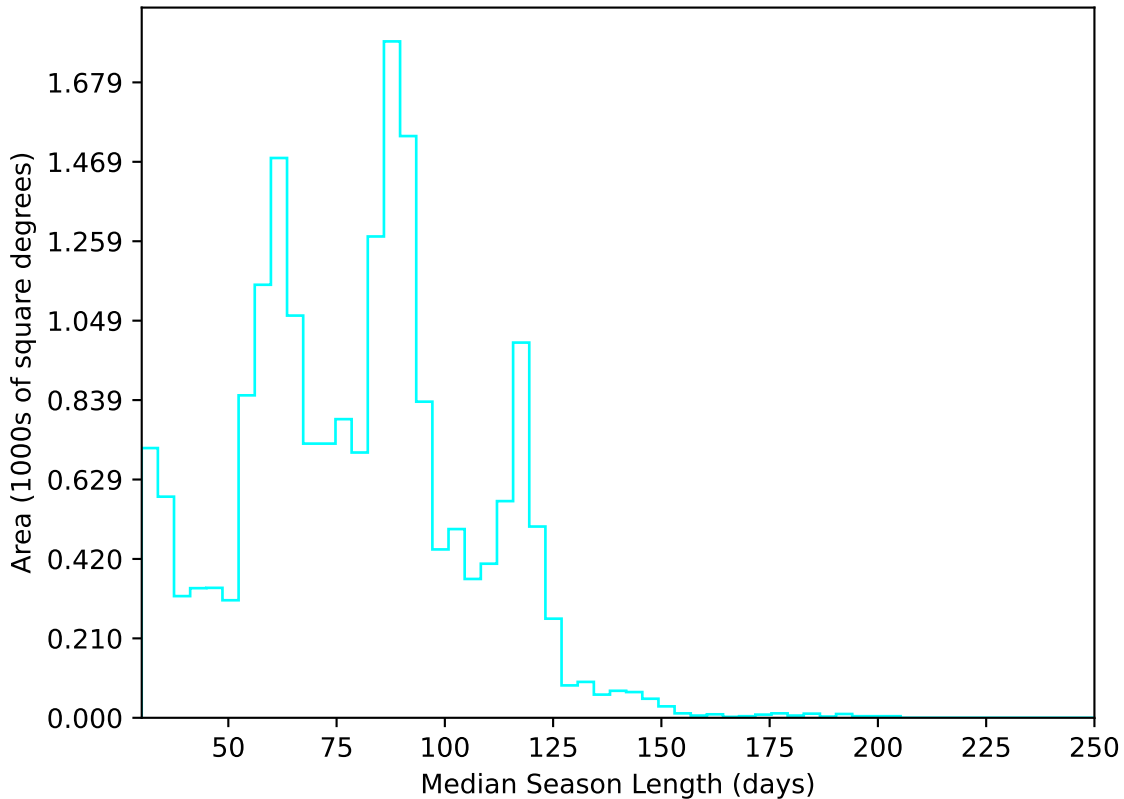
too_elab_r8_d3_ugrizy_v3.4_10yrs All sky u band: Median Season Length
