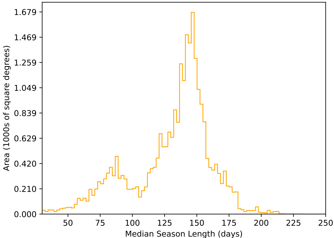
too_elab_r8_d3_ugrizy_v3.4_10yrs All sky r band: Median Season Length
