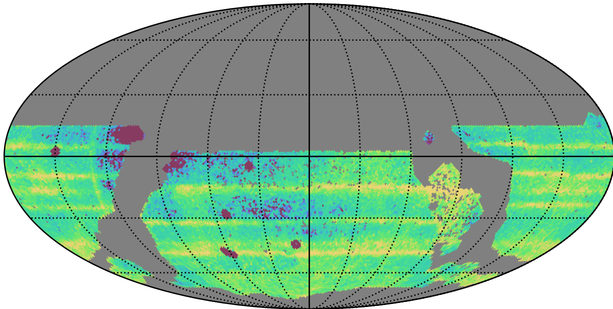
too_elab_r8_d3_ugrizy_v3.4_10yrs WFD: Median Intra-Night Gap
