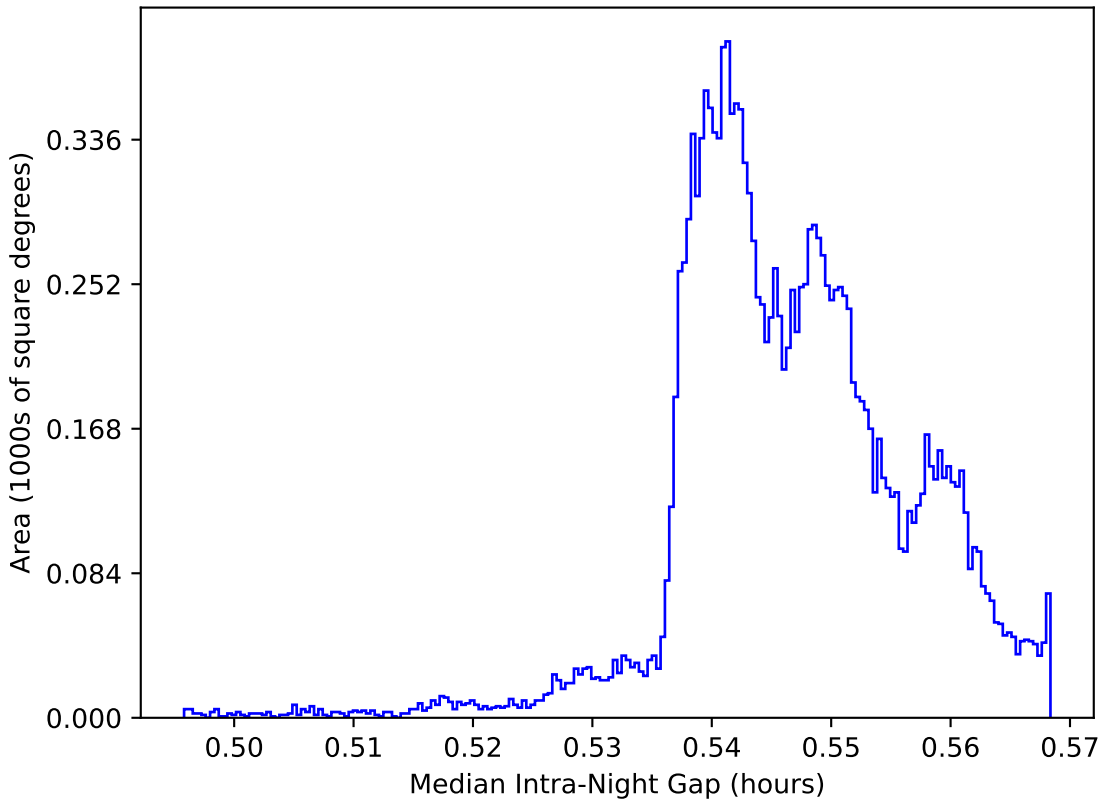
too_elab_r8_d3_ugrizy_v3.4_10yrs WFD: Median Intra-Night Gap
