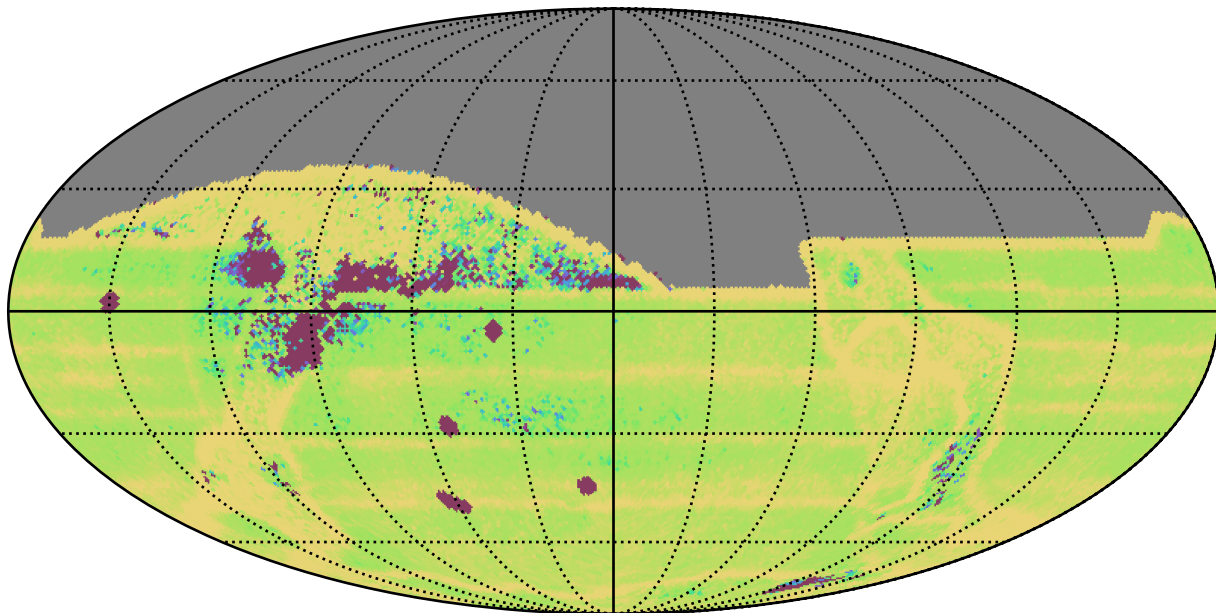
too_elab_r8_d3_ugrizy_v3.4_10yrs All sky: Median Intra-Night Gap
