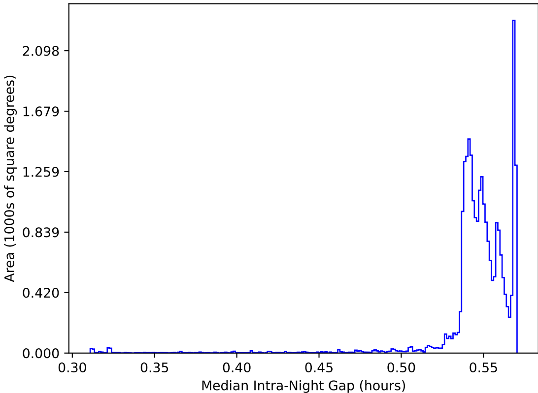
too_elab_r8_d3_ugrizy_v3.4_10yrs All sky: Median Intra-Night Gap
