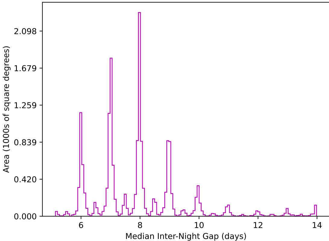
too_elab_r8_d3_ugrizy_v3.4_10yrs WFD z band: Median Inter-Night Gap
