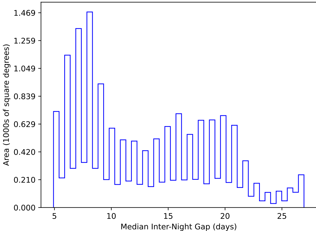
too_elab_r8_d3_ugrizy_v3.4_10yrs WFD y band: Median Inter-Night Gap
