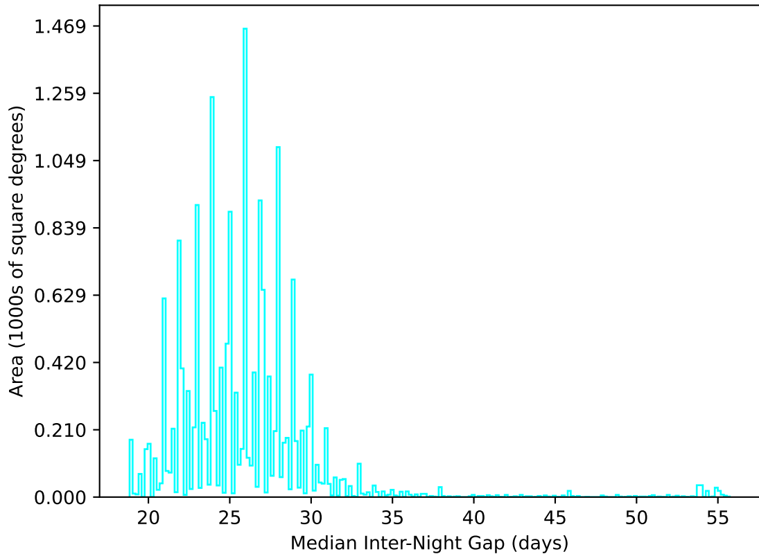
too_elab_r8_d3_ugrizy_v3.4_10yrs WFD u band: Median Inter-Night Gap
