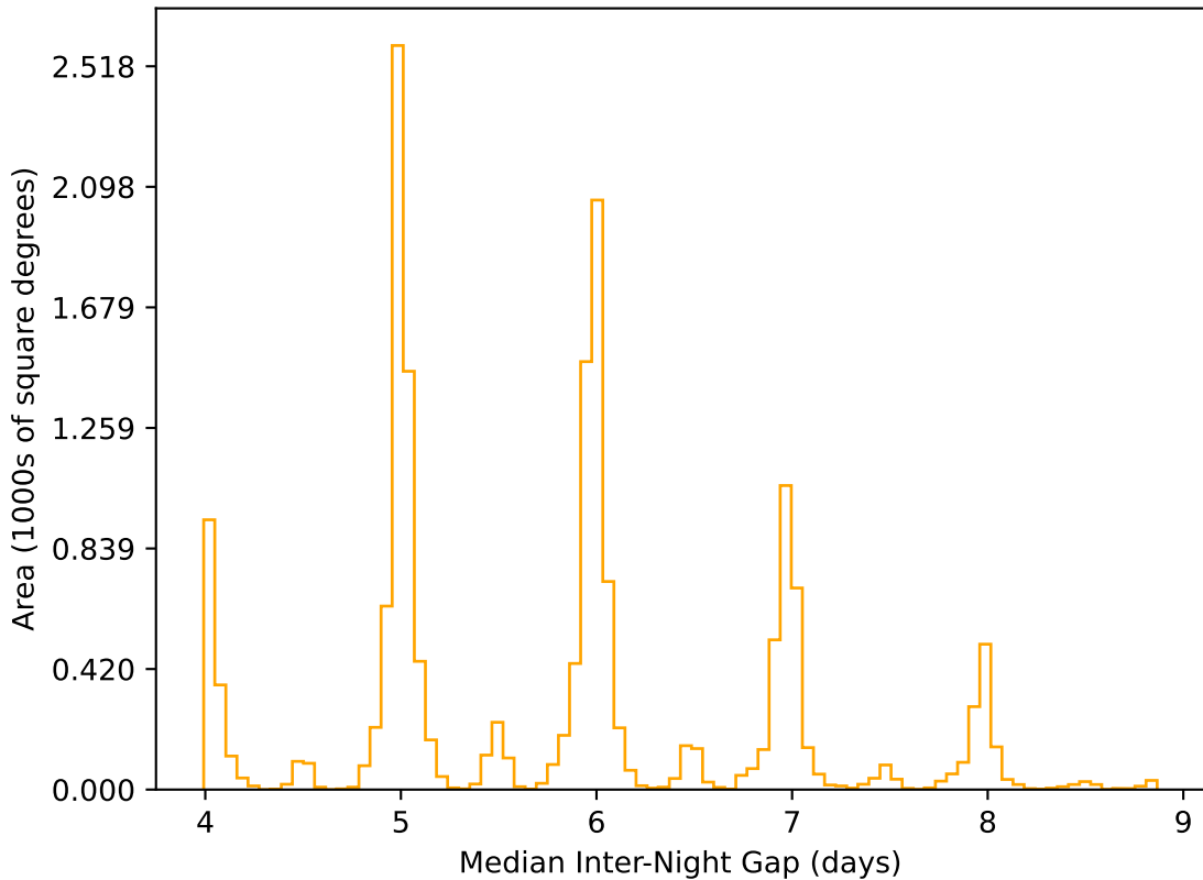
too_elab_r8_d3_ugrizy_v3.4_10yrs WFD r band: Median Inter-Night Gap
