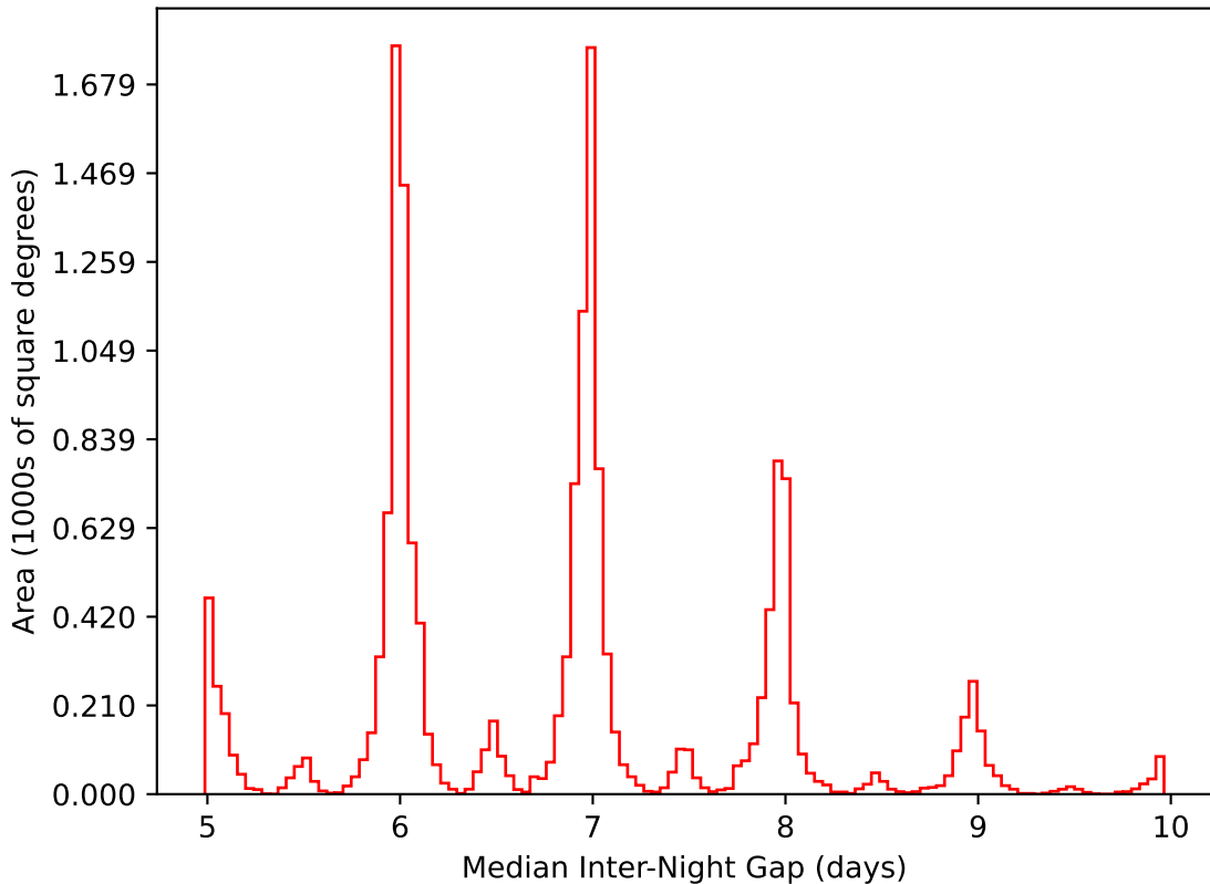
too_elab_r8_d3_ugrizy_v3.4_10yrs WFD i band: Median Inter-Night Gap
