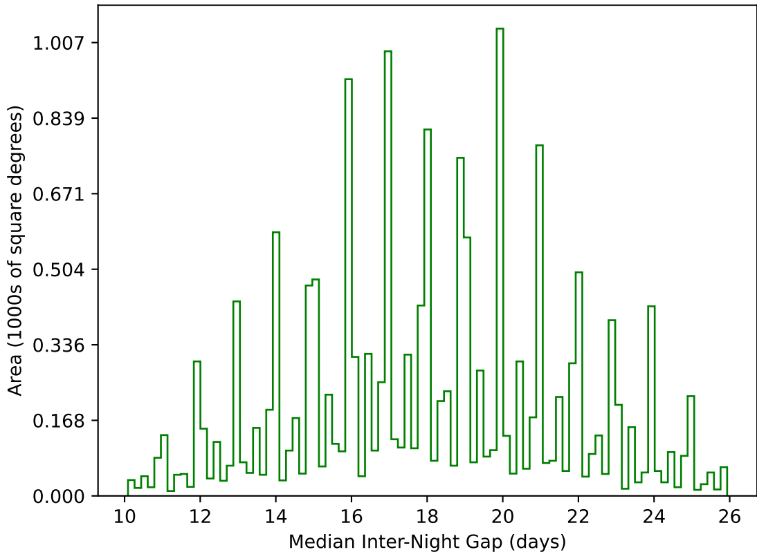
too_elab_r8_d3_ugrizy_v3.4_10yrs WFD g band: Median Inter-Night Gap
