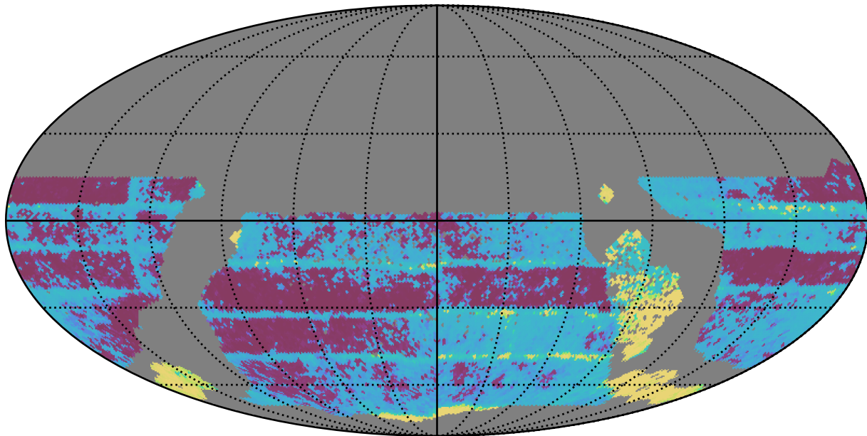
too_elab_r8_d3_ugrizy_v3.4_10yrs WFD all bands: Median Inter-Night Gap
