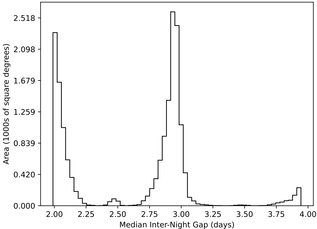
too_elab_r8_d3_ugrizy_v3.4_10yrs WFD all bands: Median Inter-Night Gap
