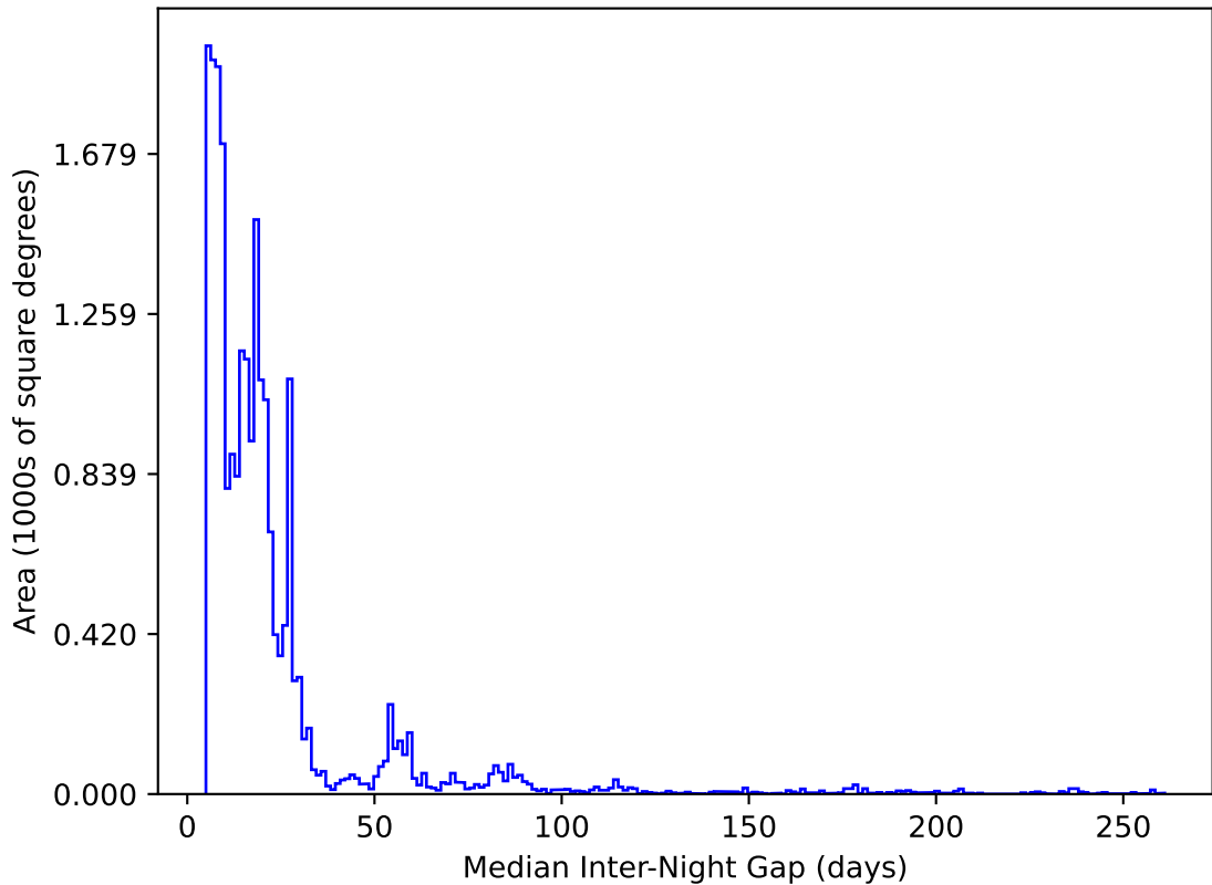
too_elab_r8_d3_ugrizy_v3.4_10yrs All sky y band: Median Inter-Night Gap
