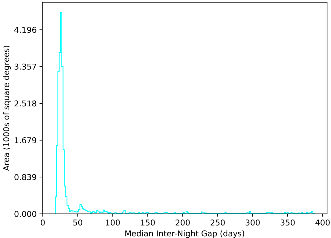
too_elab_r8_d3_ugrizy_v3.4_10yrs All sky u band: Median Inter-Night Gap
