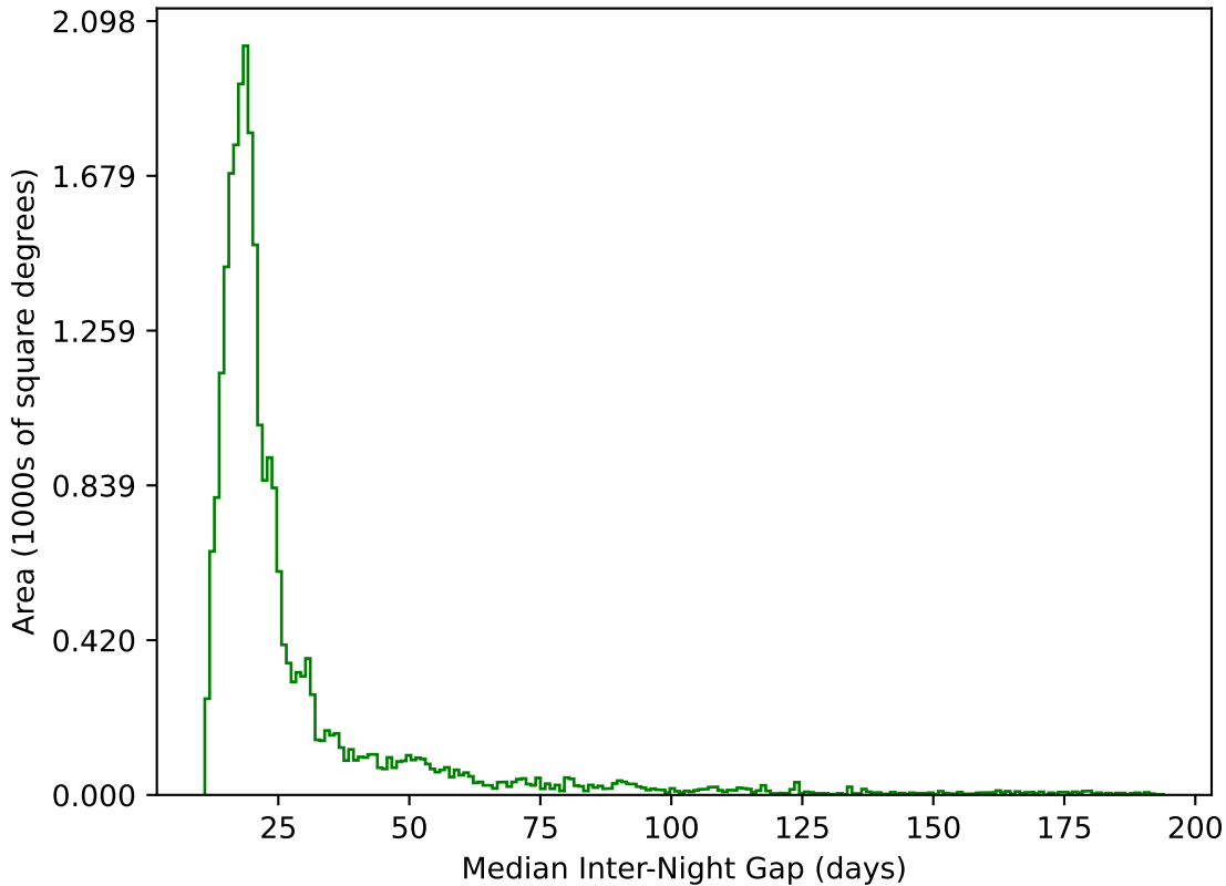
too_elab_r8_d3_ugrizy_v3.4_10yrs All sky g band: Median Inter-Night Gap
