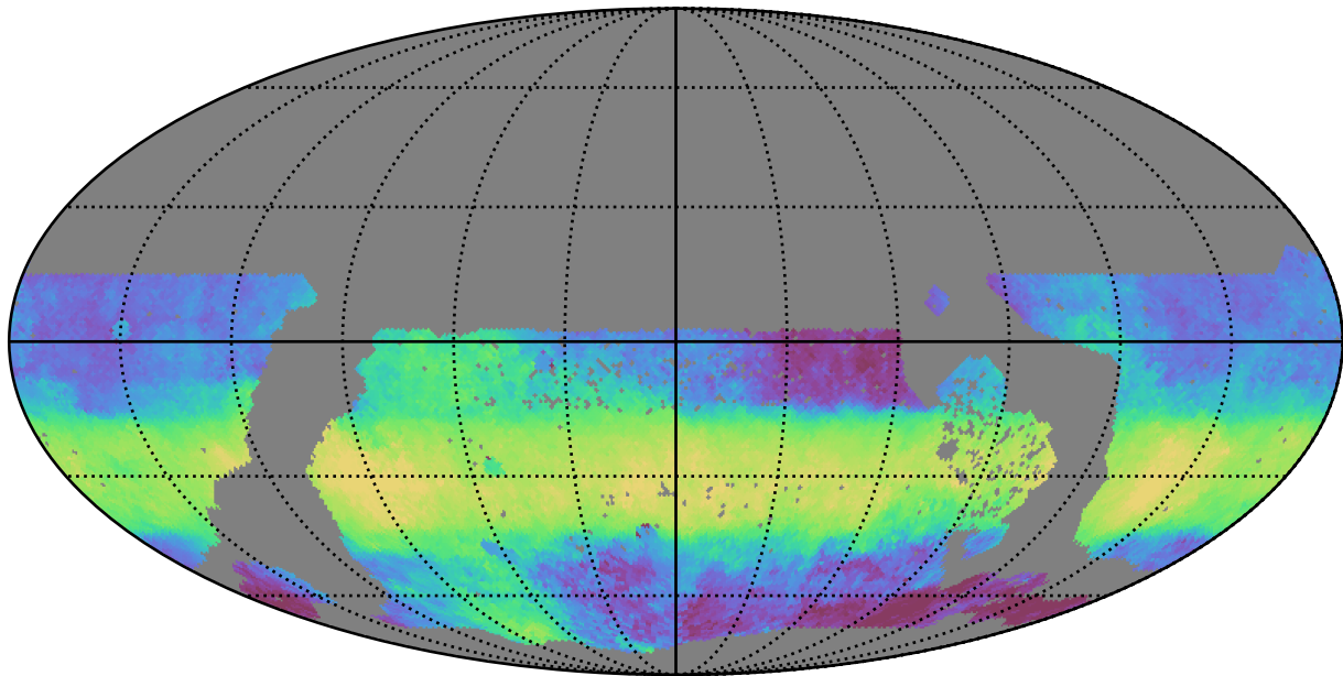
too_elab_r8_d3_ugrizy_v3.4_10yrs WFD z band: Median HA
