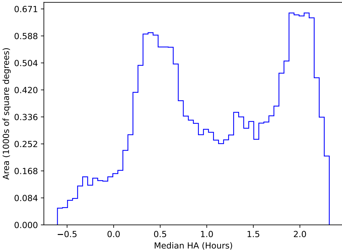
too_elab_r8_d3_ugrizy_v3.4_10yrs WFD z band: Median HA
