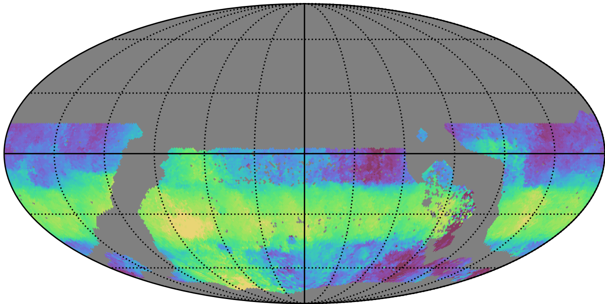
too_elab_r8_d3_ugrizy_v3.4_10yrs WFD u band: Median HA
