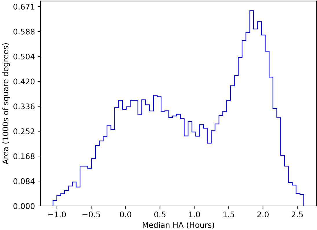
too_elab_r8_d3_ugrizy_v3.4_10yrs WFD u band: Median HA
