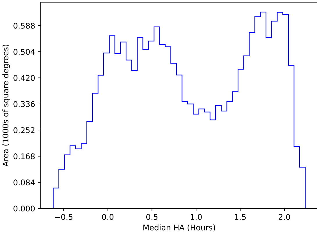
too_elab_r8_d3_ugrizy_v3.4_10yrs WFD r band: Median HA
