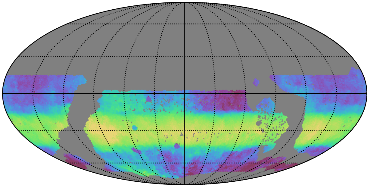
too_elab_r8_d3_ugrizy_v3.4_10yrs WFD i band: Median HA
