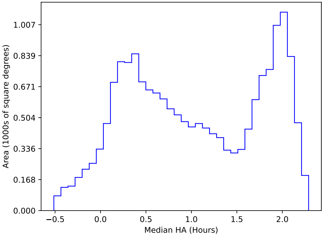
too_elab_r8_d3_ugrizy_v3.4_10yrs WFD i band: Median HA
