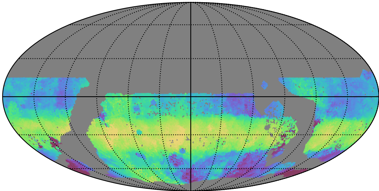
too_elab_r8_d3_ugrizy_v3.4_10yrs WFD g band: Median HA
