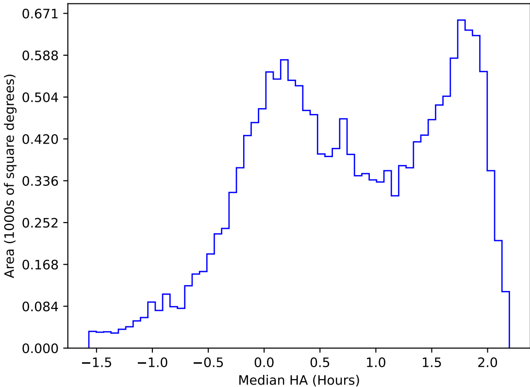
too_elab_r8_d3_ugrizy_v3.4_10yrs WFD g band: Median HA
