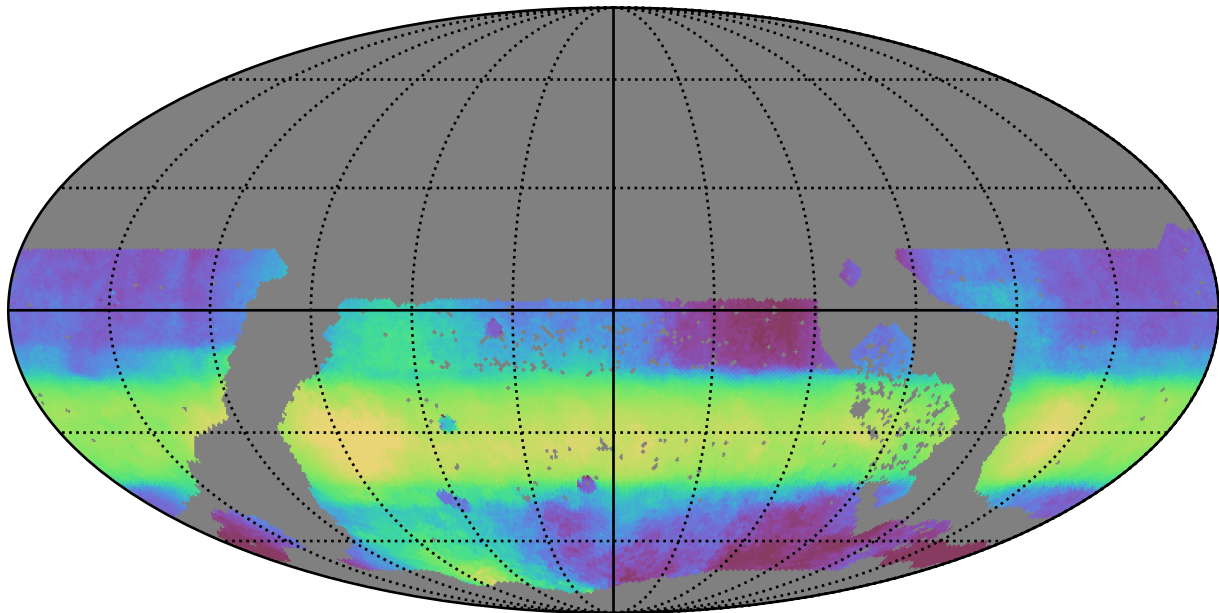
too_elab_r8_d3_ugrizy_v3.4_10yrs WFD all bands: Median HA
