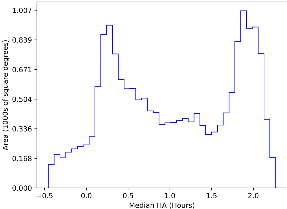
too_elab_r8_d3_ugrizy_v3.4_10yrs WFD all bands: Median HA
